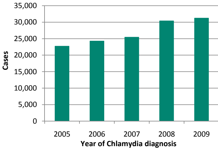
Figure 6. Chlamydia cases, 2005-2009
