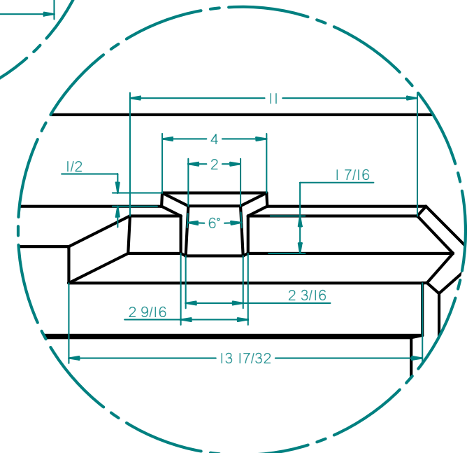
DETAIL H
