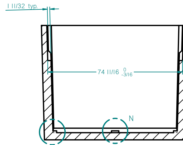
SECTION K-K
