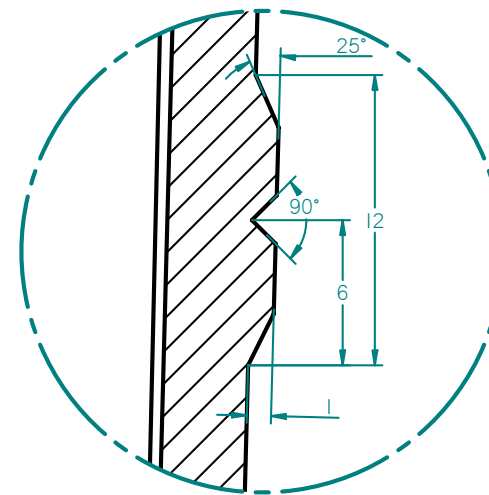
DETAIL L (Outside lifting groove)
