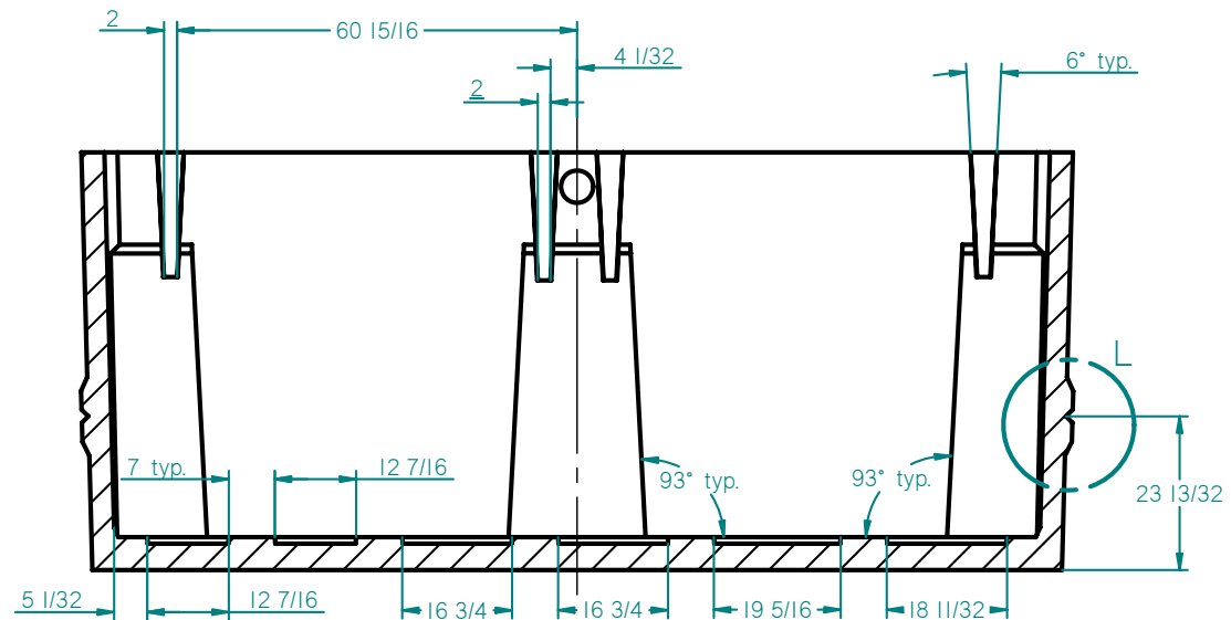
SECTION J-J
