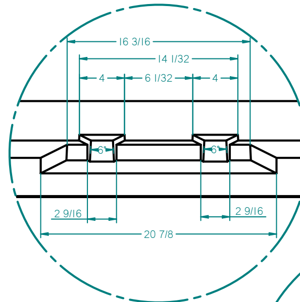
DETAIL G
