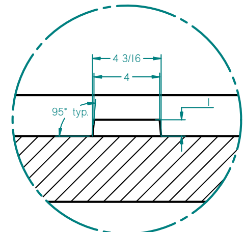
DETAIL N
