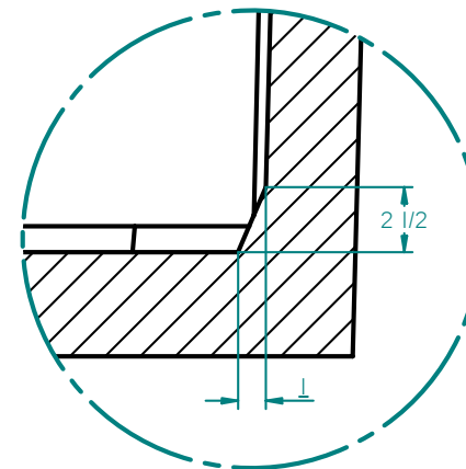
DETAIL I
