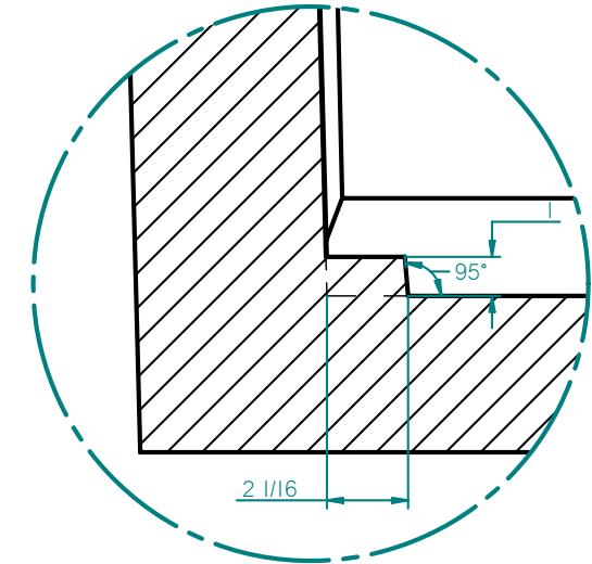
DETAIL M
