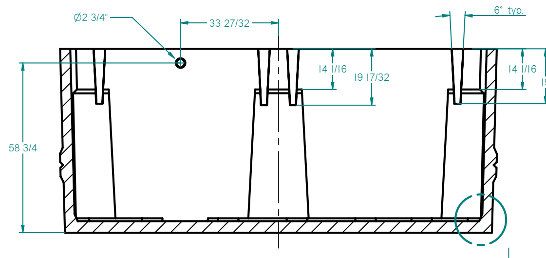
SECTION F-F
