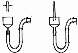
Air Gap
